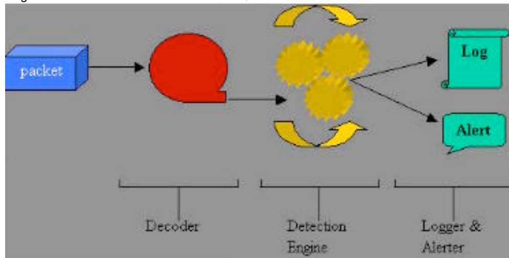
Figure 3: Snort Architecture.
